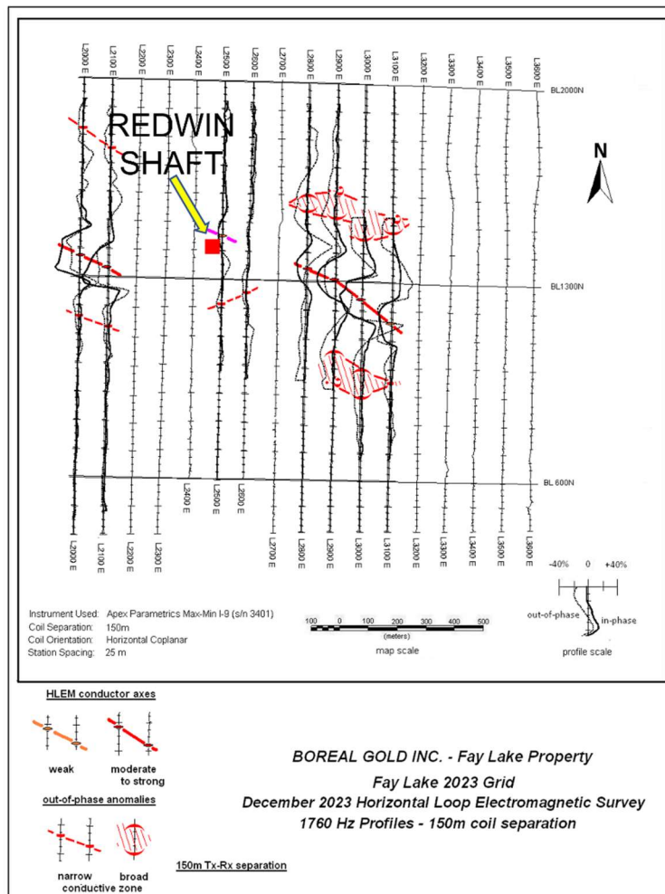
Figure 25: HLEM Survey on the Redwin Peninsula area showing the location of HLEM conductors in relationship to the Redwin Shaft area. The HLEM profiles are from the survey carried out at 1760 Hz with 150 coil separation.
